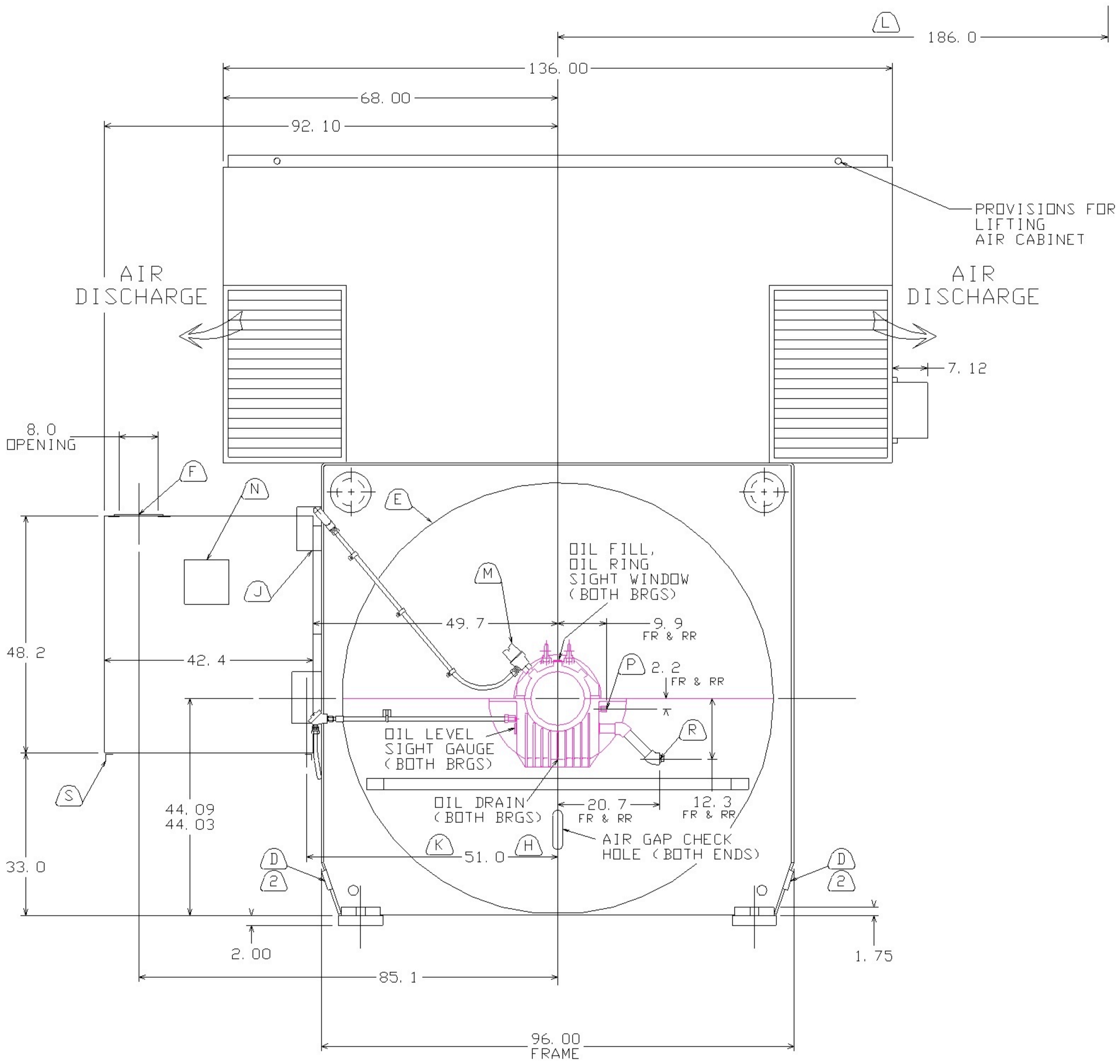
FRONT VIEW
